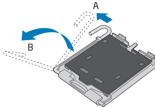
Figure 6. Lift the Socket Lever
